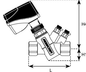
FlowCon Green.0/1 in FlowCon AB valve DN15/20/25 (1/2", 3/4", 1") w. FlowCon FN.0.2-BUS, FN.0.4 + FNP.0.2 actuator
